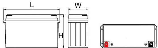
Dimensional diagram
