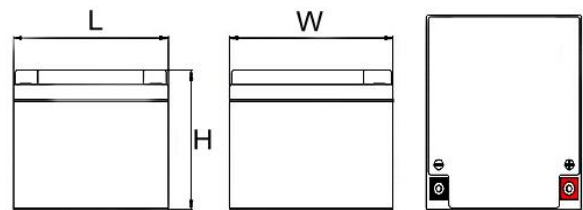
Dimensional diagram
