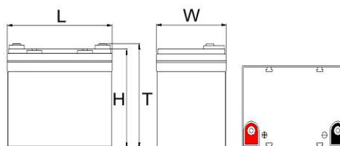
Dimensional diagram
