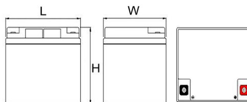
Dimensional diagram
