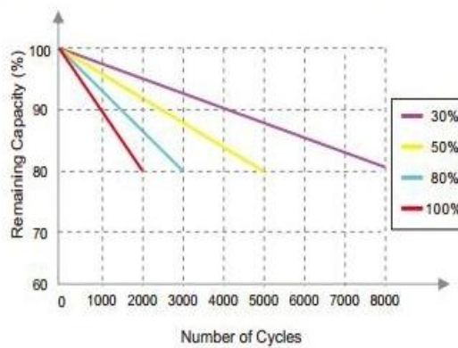
Different DOD Discharge Cycle Life Curve @1C
