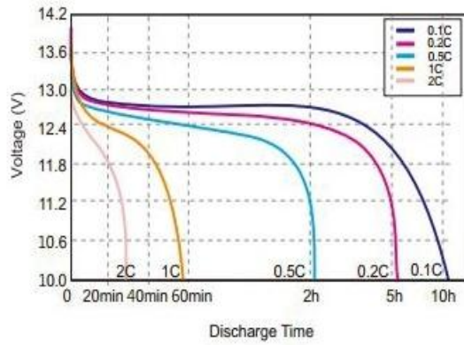
Different Rate Discharge Curve @25°C
