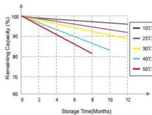
Different Temperature Self Discharge Curve
